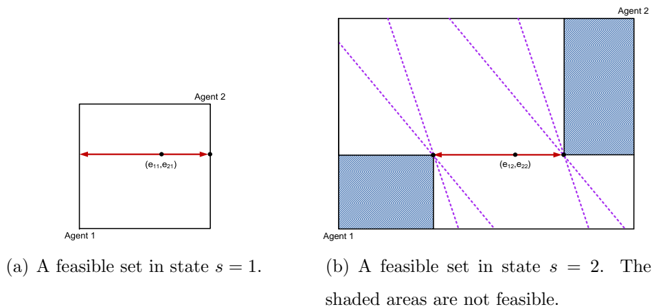
Figure 1: Feasible Sets in state s = 1 and s = 2 when markets are incomplete. The only available security pays the same amount of good 1 in both states.
